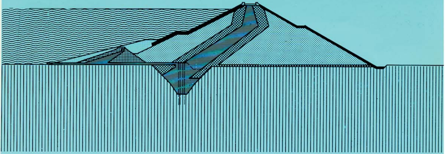
Dam cross section
